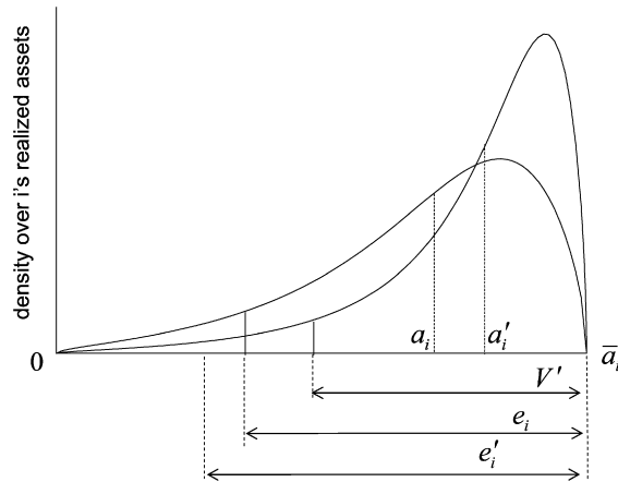
Fig. 2. Economic capital and market equity.
