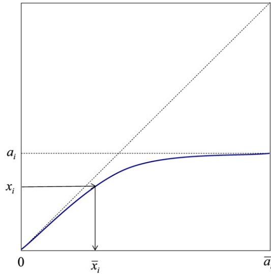
Fig. 3. Determination of \bar{x}_i given x_i and a_i .
